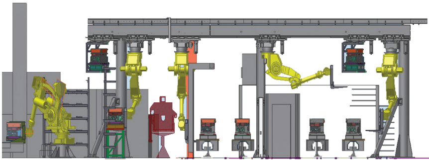
GANTRY ROBOT & ROBOTIC CELL
