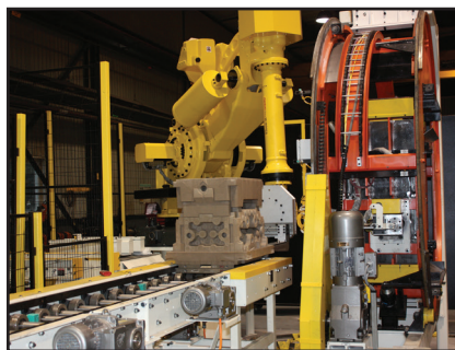
ENGINE BLOCK ROBOTIC HANDLING SYSTEM
